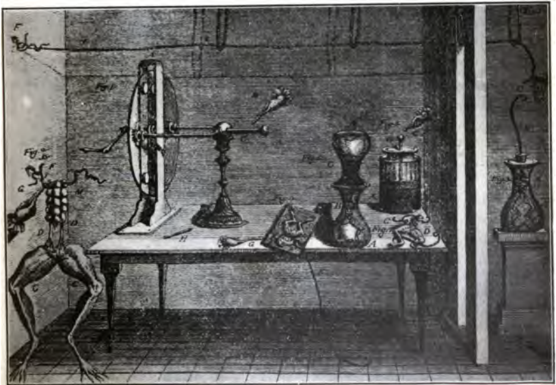
SOME OF GALVANI'S EXPERIMENTS WITH FROGS' LEGS AS DEPICTED IN HIS ORIGINAL COMMUNICATION Digitized by Google (Facing page 82)
